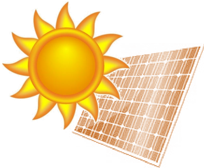
Solar electricity
